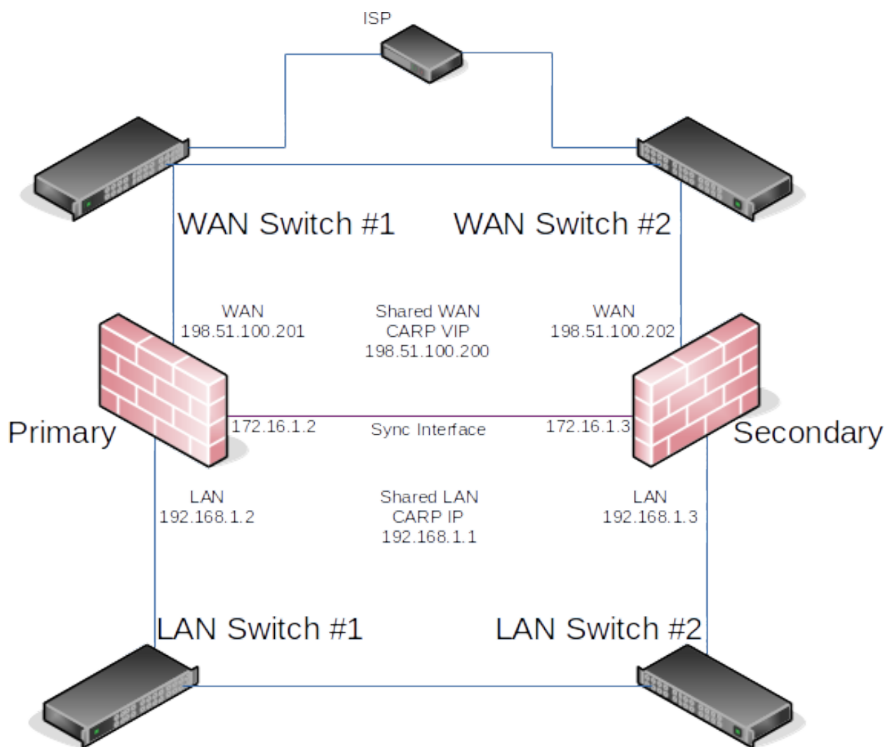
Fig. 2: Diagram of HA with Redundant Switches
