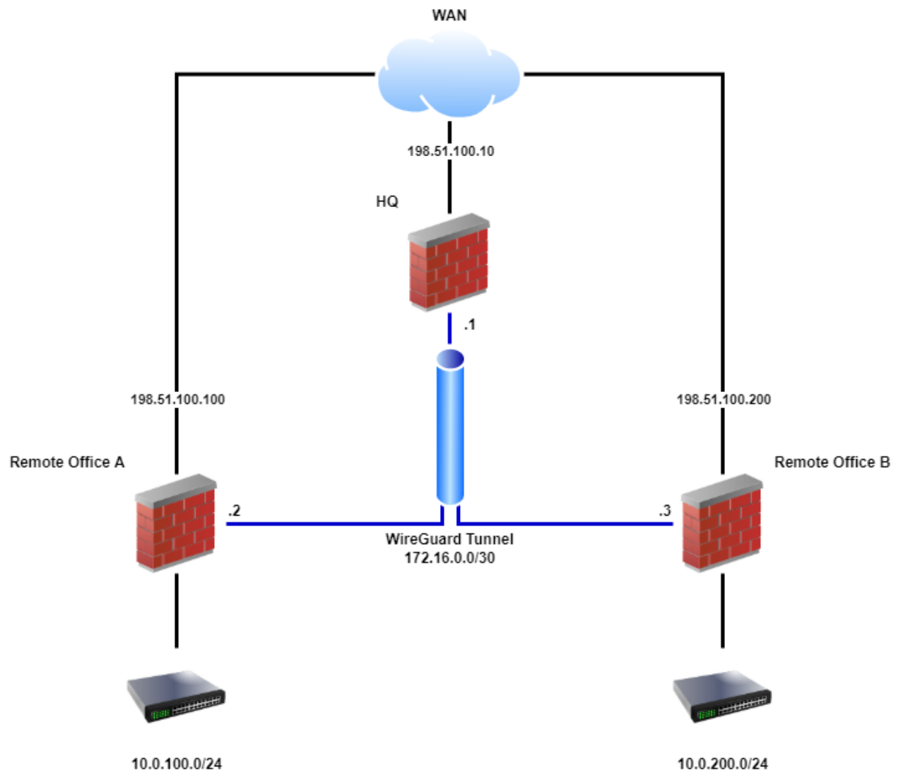
Fig. 84: WireGuard Example Site-to-Multisite Network
