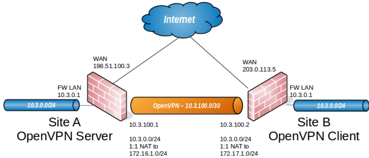
Fig. 79: Site to Site with Conflicting Subnets
