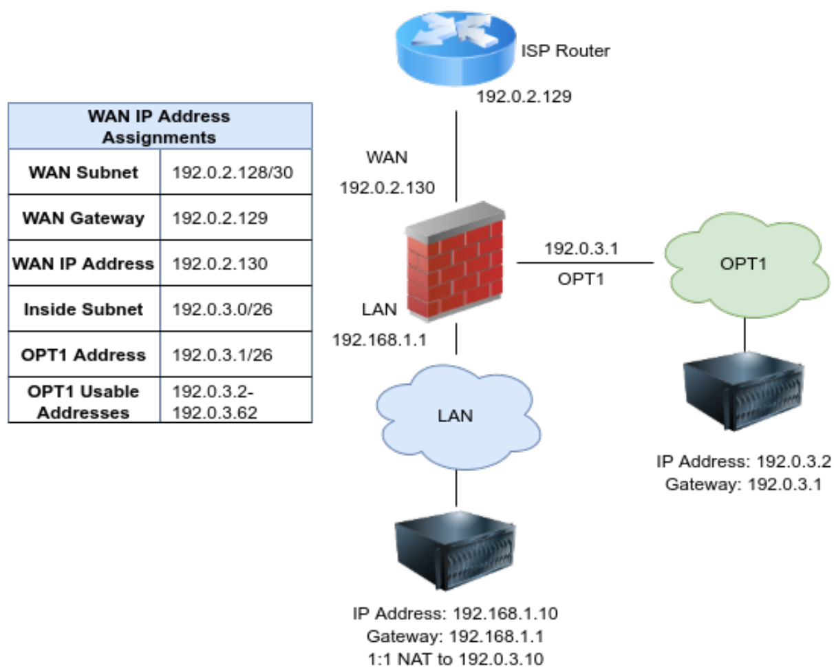
Fig. 19: Multiple Public IP Addresses Using Two IP Subnets
