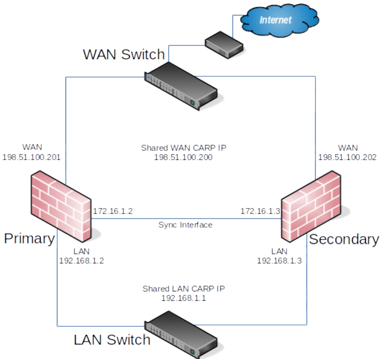
Fig. 5: Example HA Network Diagram
