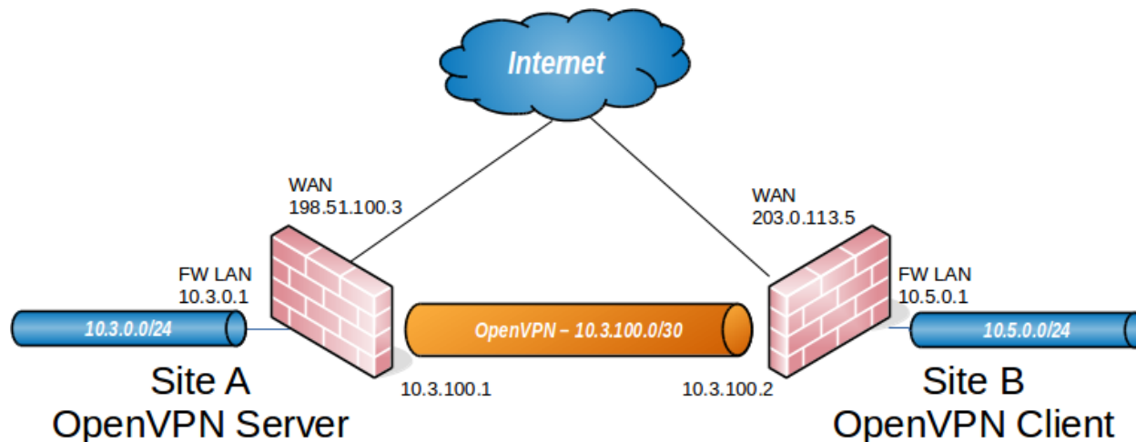
Fig. 68: OpenVPN Example Site-to-Site Network
