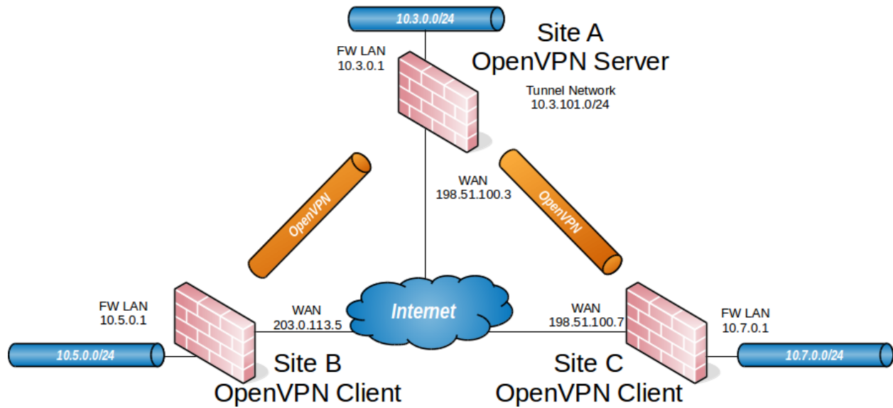
Fig. 67: OpenVPN Example Site-to-Site SSL/TLS Network
