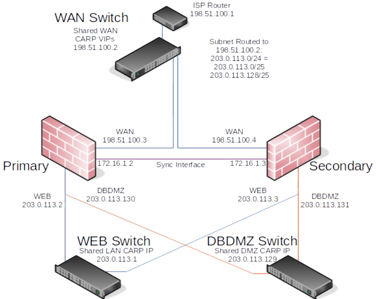
Fig. 10: Diagram of HA with Routed IPs
