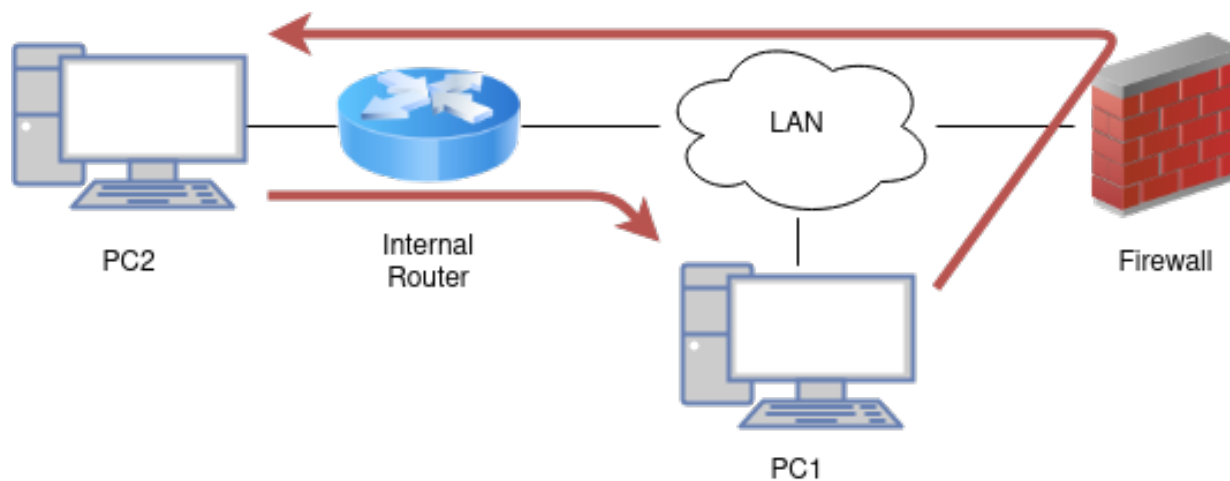
Fig. 3: Asymmetric Routing
