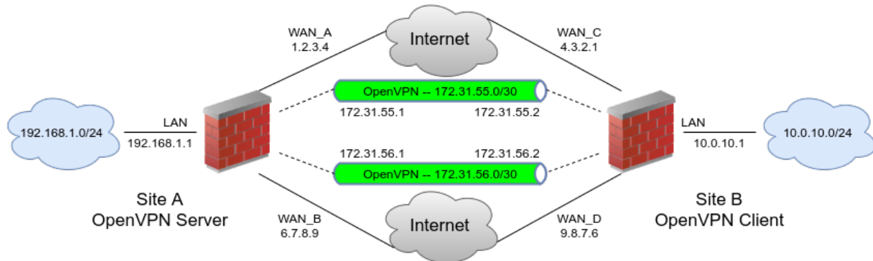
Fig. 82: Example OpenVPN Setup Involving OSPF Across Multiple WANs
