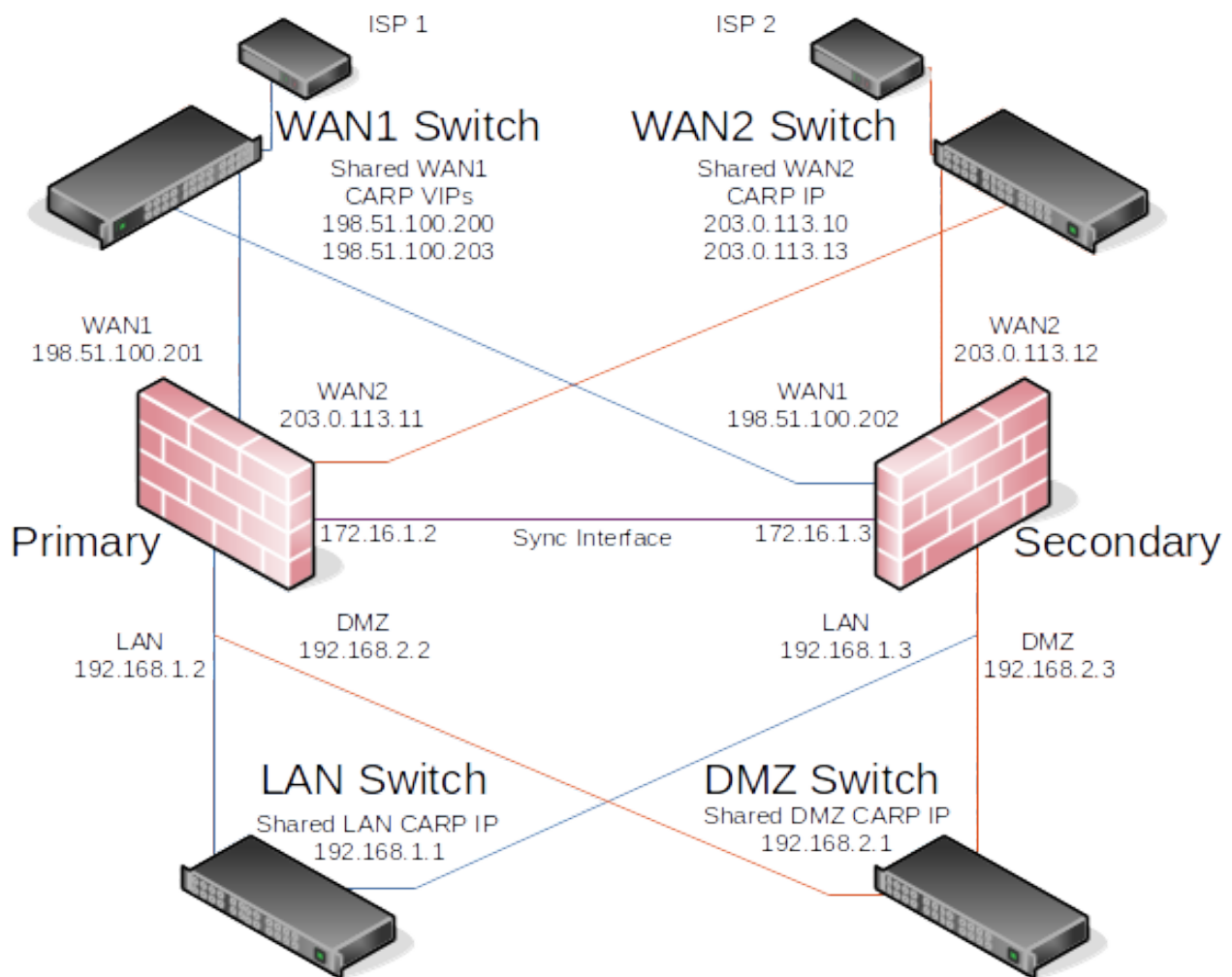
Fig. 9: Diagram of Multi-WAN HA with DMZ
